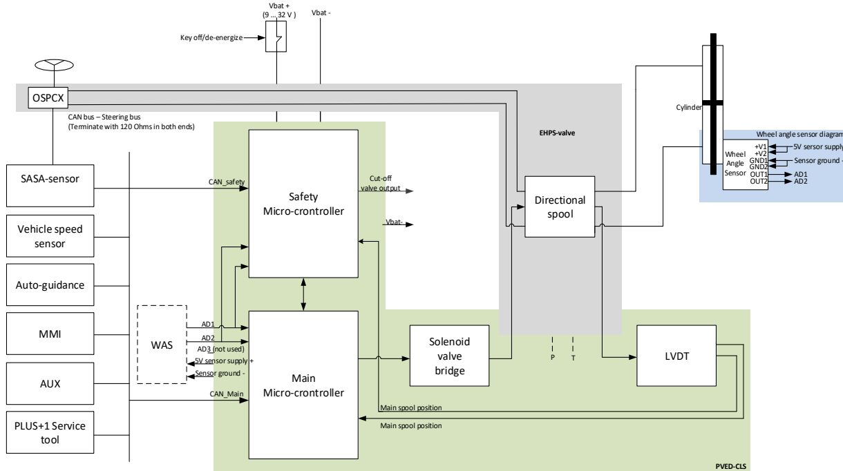
Figure 4 EHPS System
