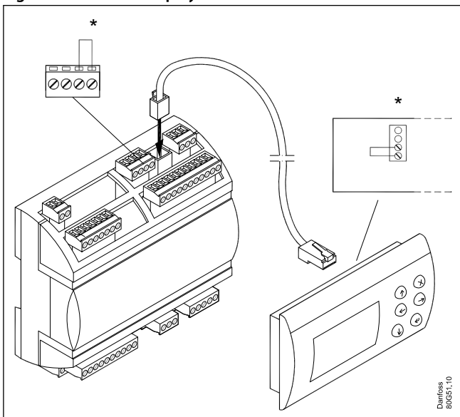
Figure 28: External display
