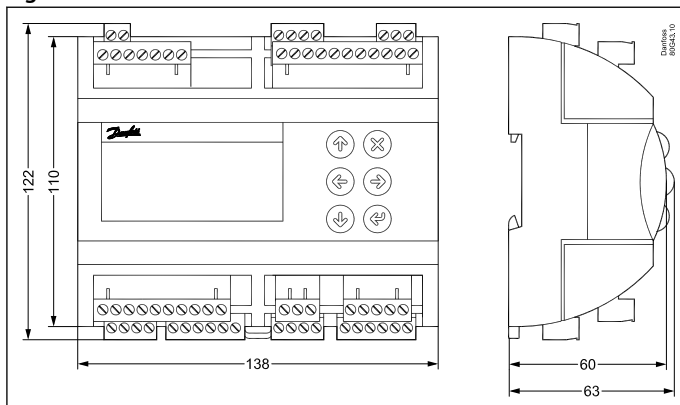
Figure 29: Dimensions
