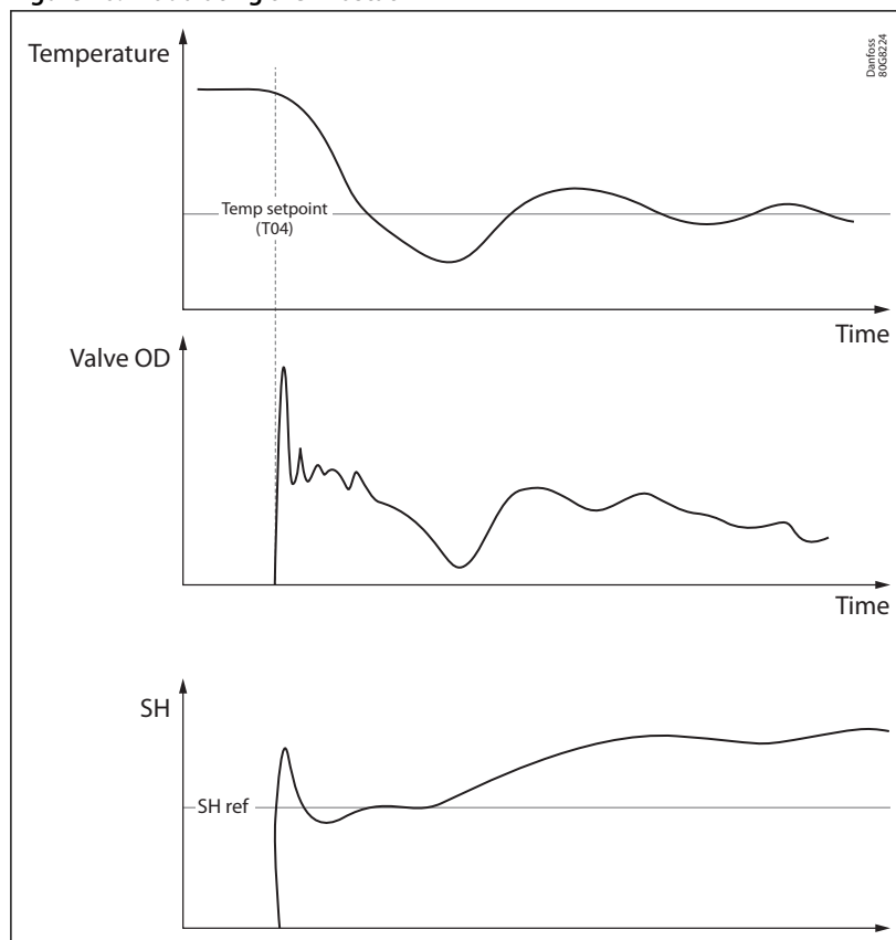
Figure 10: Modulating thermostat
