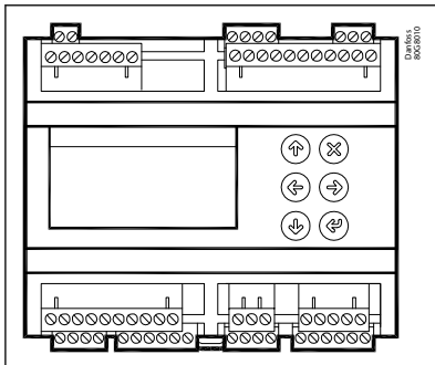
Figure 7: EKE 400
