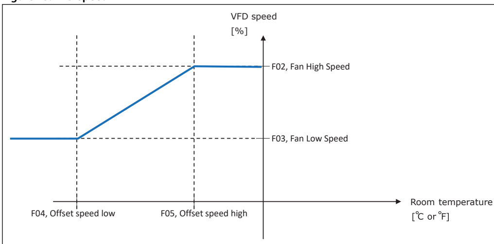
Figure 23: VFD speed
