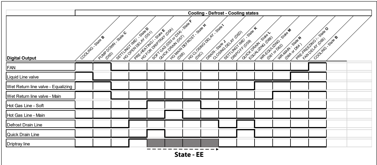
Figure 21: Defrost sequence
