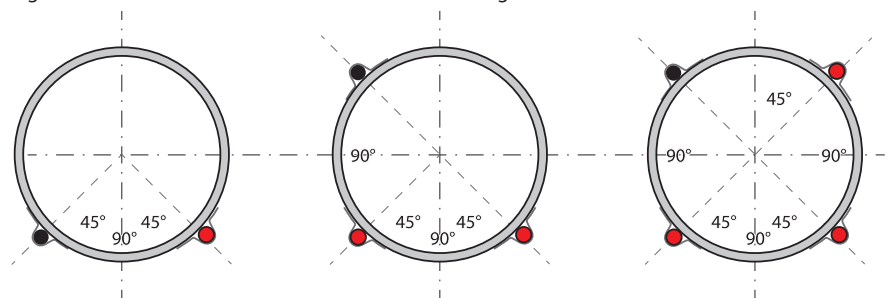
Fig. 12. Recommended ways to mount the cable lines.
