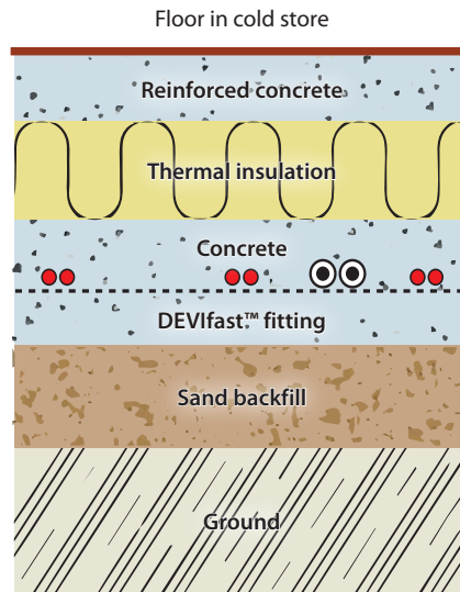
Fig. 1 – Heating cable in in the concrete screed
