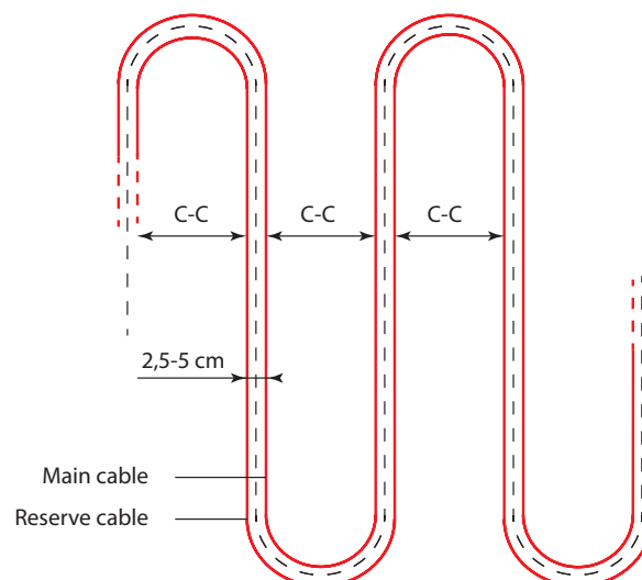
Fig. 4 – Main and reserve heating cables
