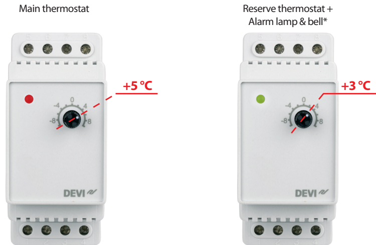
Fig. 5 – Main and reserve thermostats with settings
