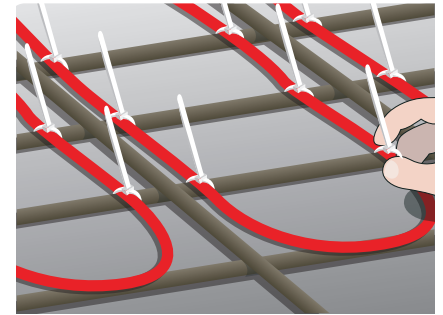
Cable ties For use on reinforcement mesh. Do NOT fix the loop. The cable must be able to move.
