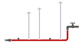
Fig 3. Without automatic differential pressure controllers, the distribution of water shows irregularities in partial load conditions.
